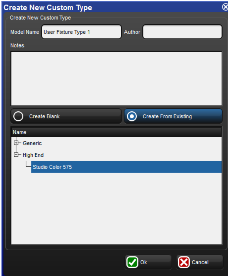
Figure 25.2. The Create New Custom Type window
